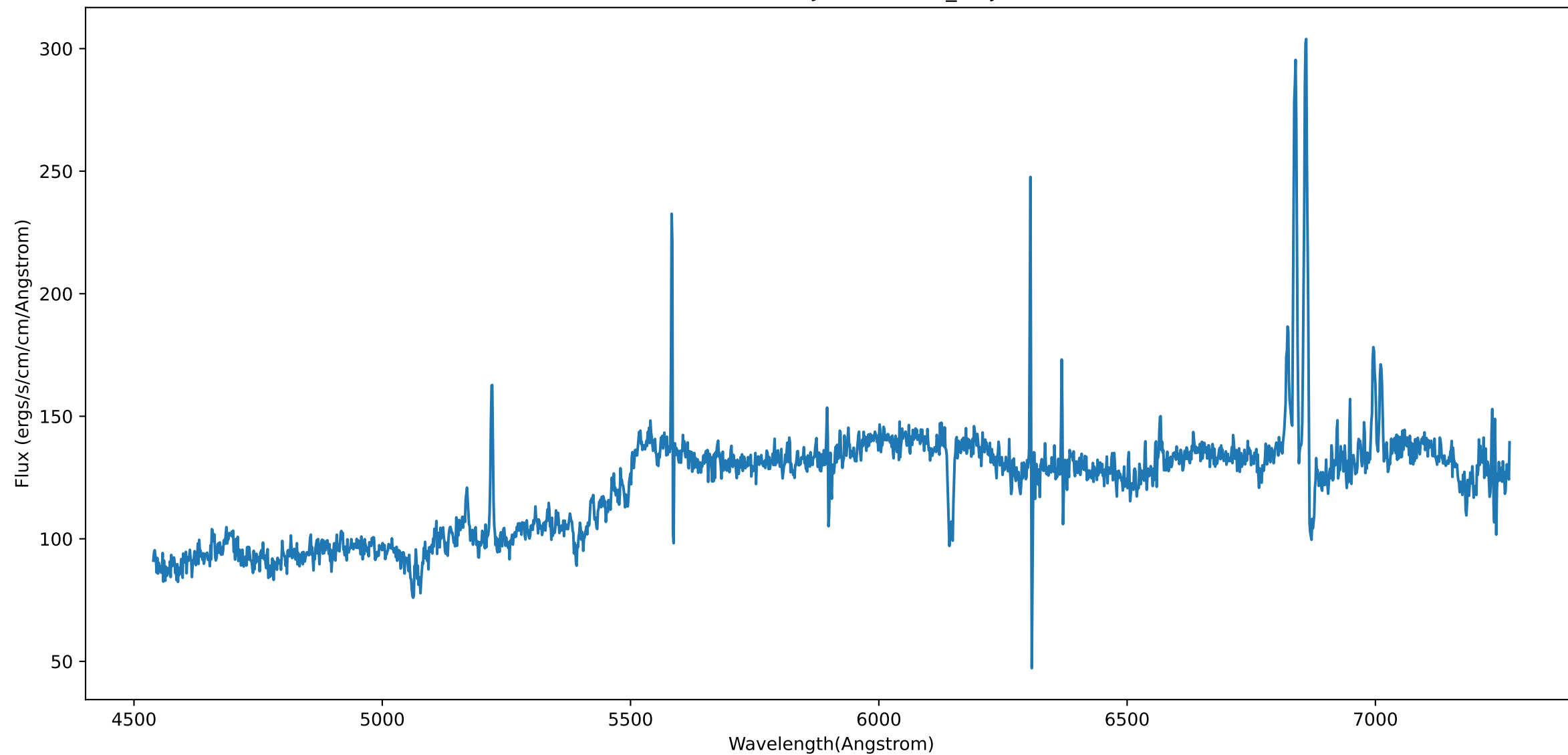
Flux Calibrated J0800+3743_major
